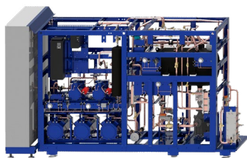
MiniCO 2 OL® Compact with integrated High Efficiency Module
