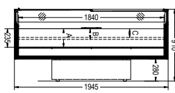
visiCUBE® TOP 200 (Front view)
