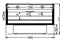
visiCUBE® TOP 150 (Front view)
