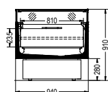
visiCUBE® TOP (Side view)
